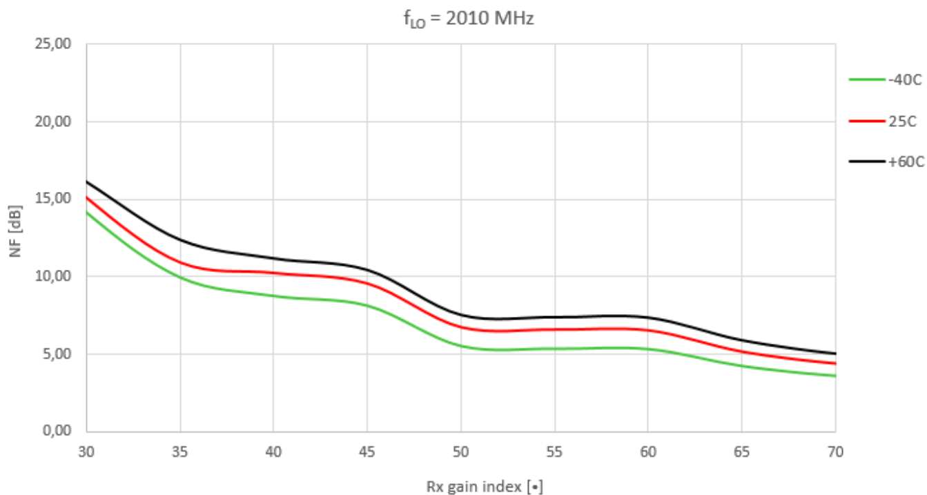
Figure 9: NF measurement while running with LO = 2010 MHz, S-band applications.
